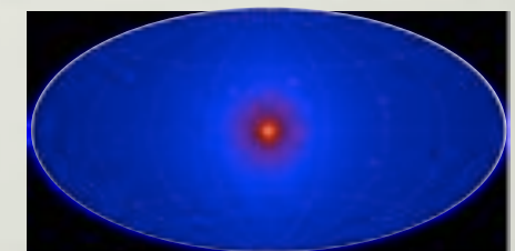
dark matter??
