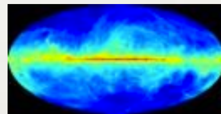
galactic diffuse
