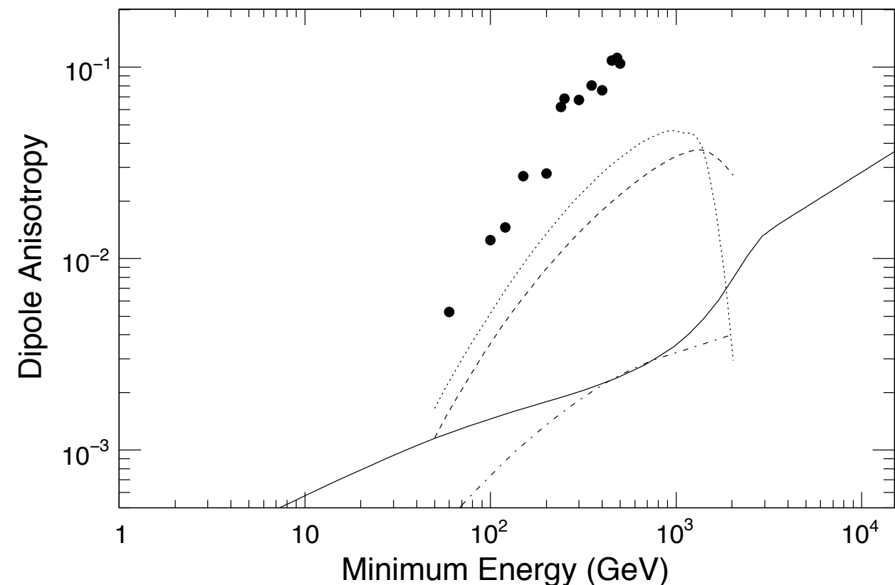
CRE dipole anisotropy limits and predictions for some DM scenarios
